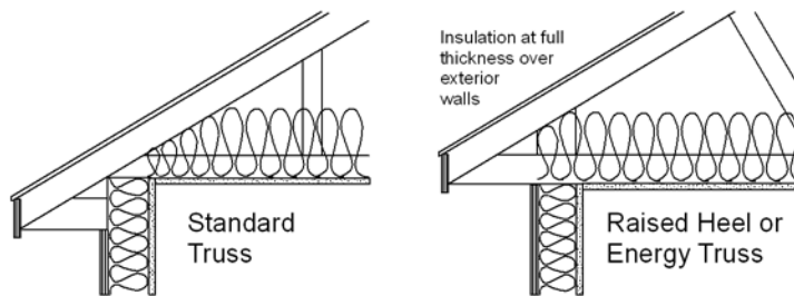
Roof Truss Insulation
